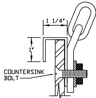
SECTION D DROP PLATE BRACKET 14 GA. STAINLESS STEEL
