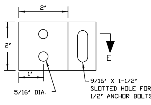
PARTITION PLATE BRACKET 12 GA. STAINLESS STEEL
